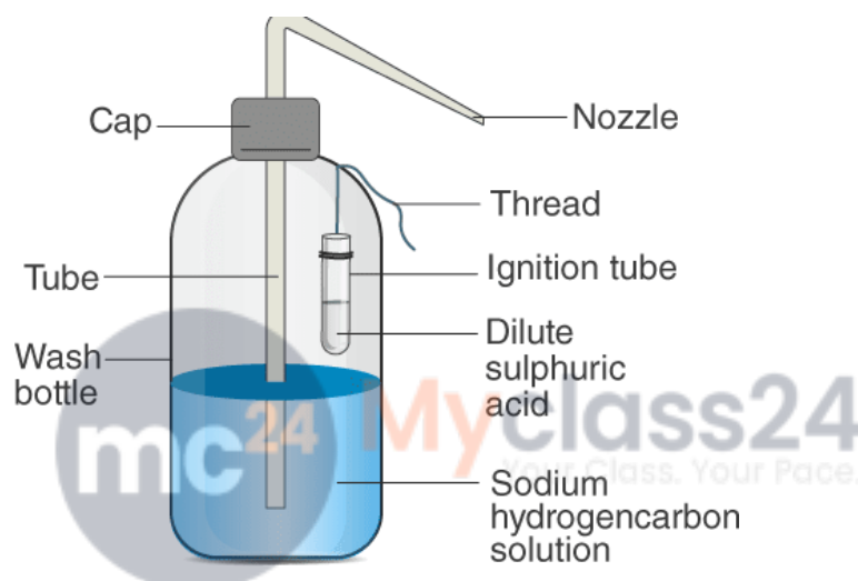
Making a soda-acid fire extinguisher
